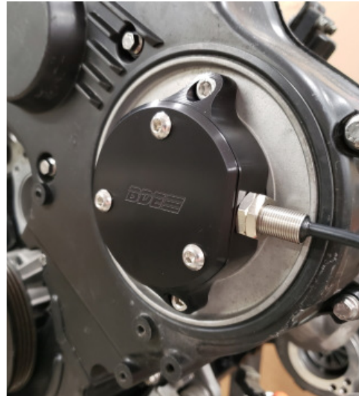
FIGURE 18 - cam sync housing cover installed
